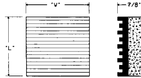
SERIES "NNP" RIBBED NEOPRENE ISOLATION PAD
