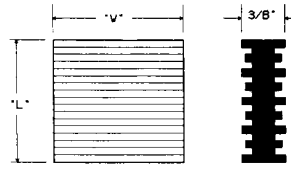
SERIES "NNP" RIBBED NEOPRENE ISOLATION PAD
